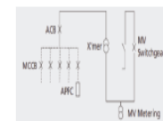
CSS MV Switchgear & Metering, ACB as I/c & MCCB as O/G with APFC
